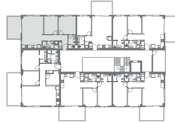
A-B-C BLOCK
