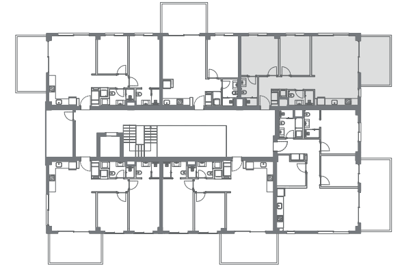
D-E-F BLOCK
